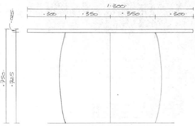
SHORT SIDE ELEVATION.
