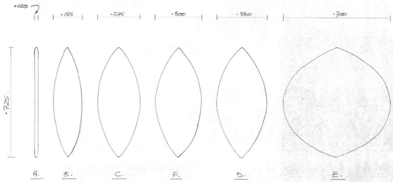
PROFILES THROUGH BASE AT POSITIONS MARKED ON PLAN
