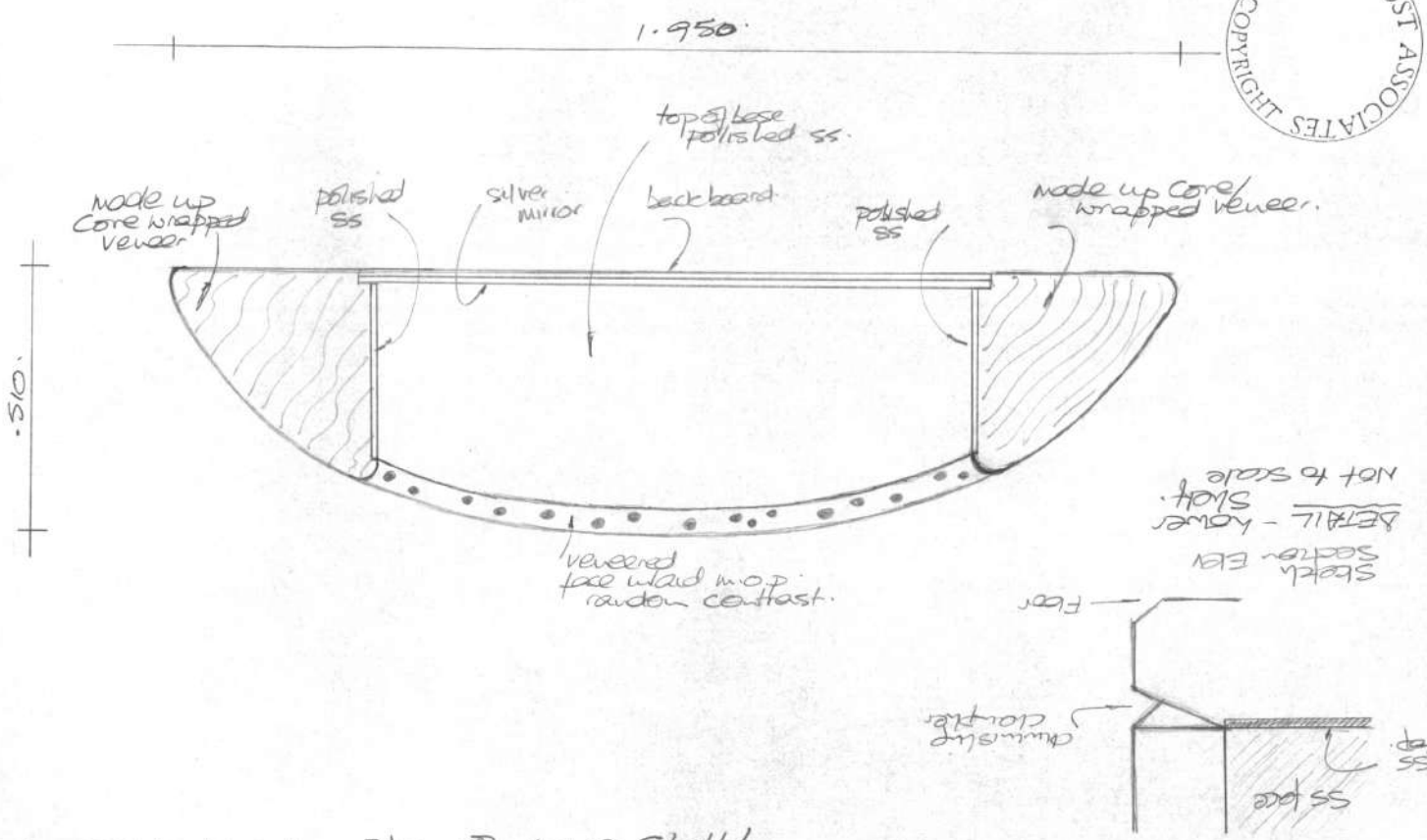
Sapa Table 4and. - Plan of lower slot / section thru' leg cores
