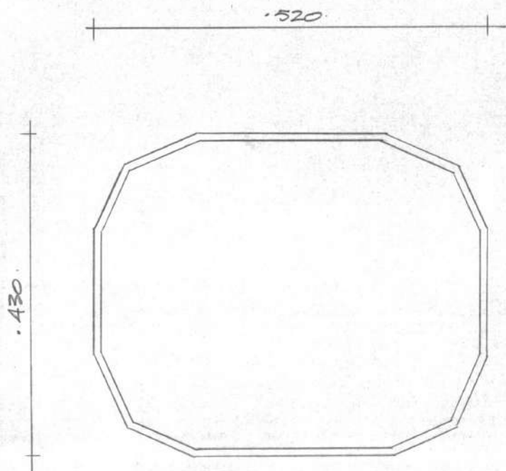
PLAN - STONE TOPS Scale 1:5.
