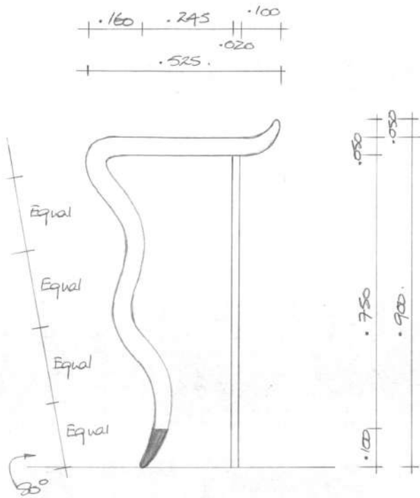
SIDE ELEVATION
