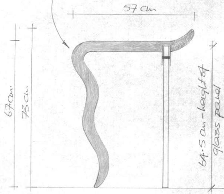
SIDE ELEVATION/SECTION
