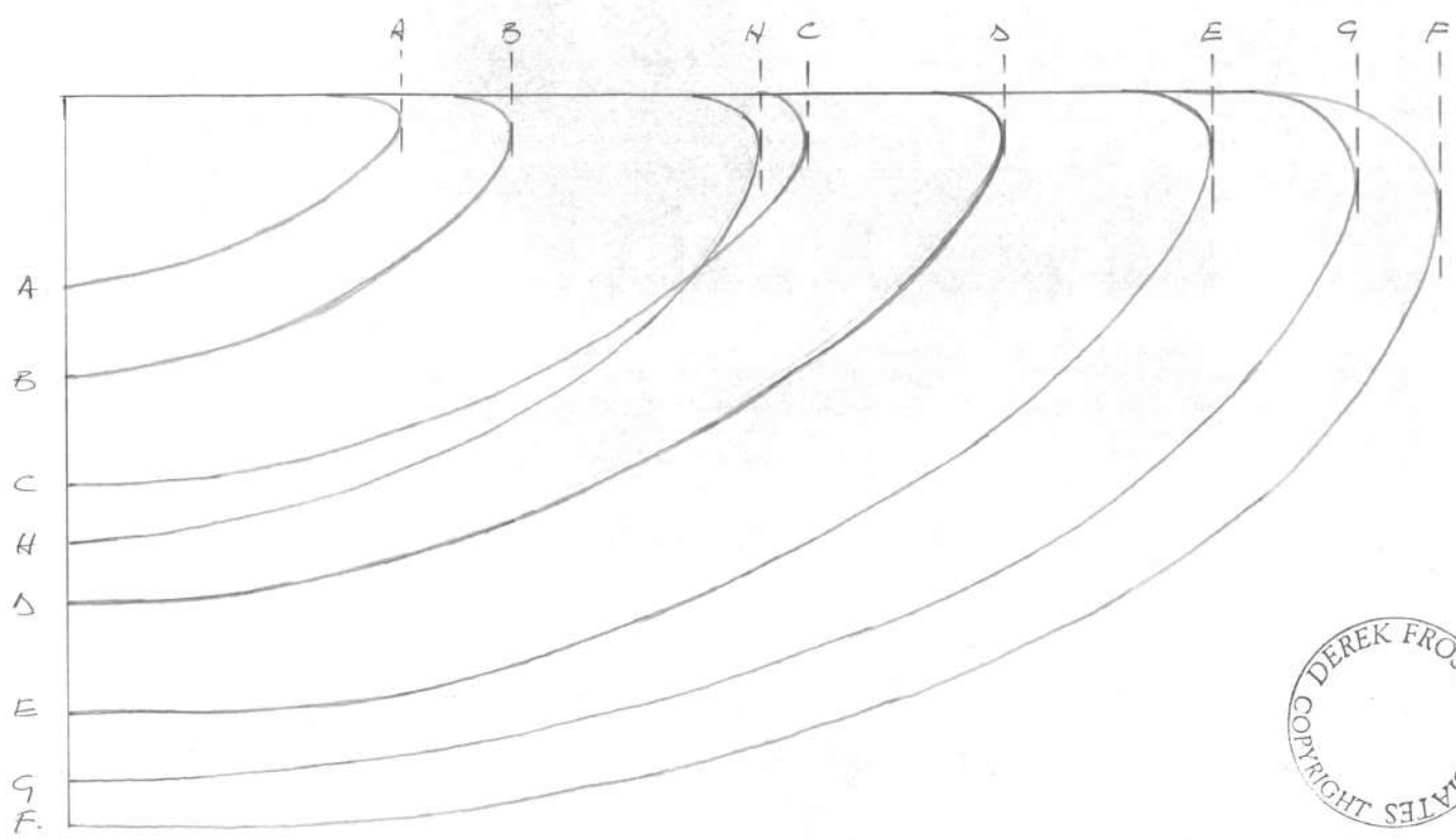
SECTIONS TO SHOW PROFILE THROUGH TERRAZZO CANTILEVER SHELF FOR THE LIBRARY BUTE HOUSE.
