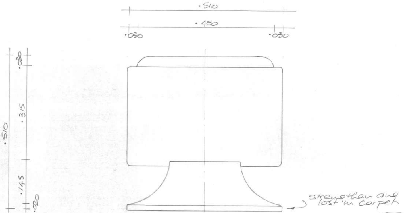
SIDE ELEVATION
