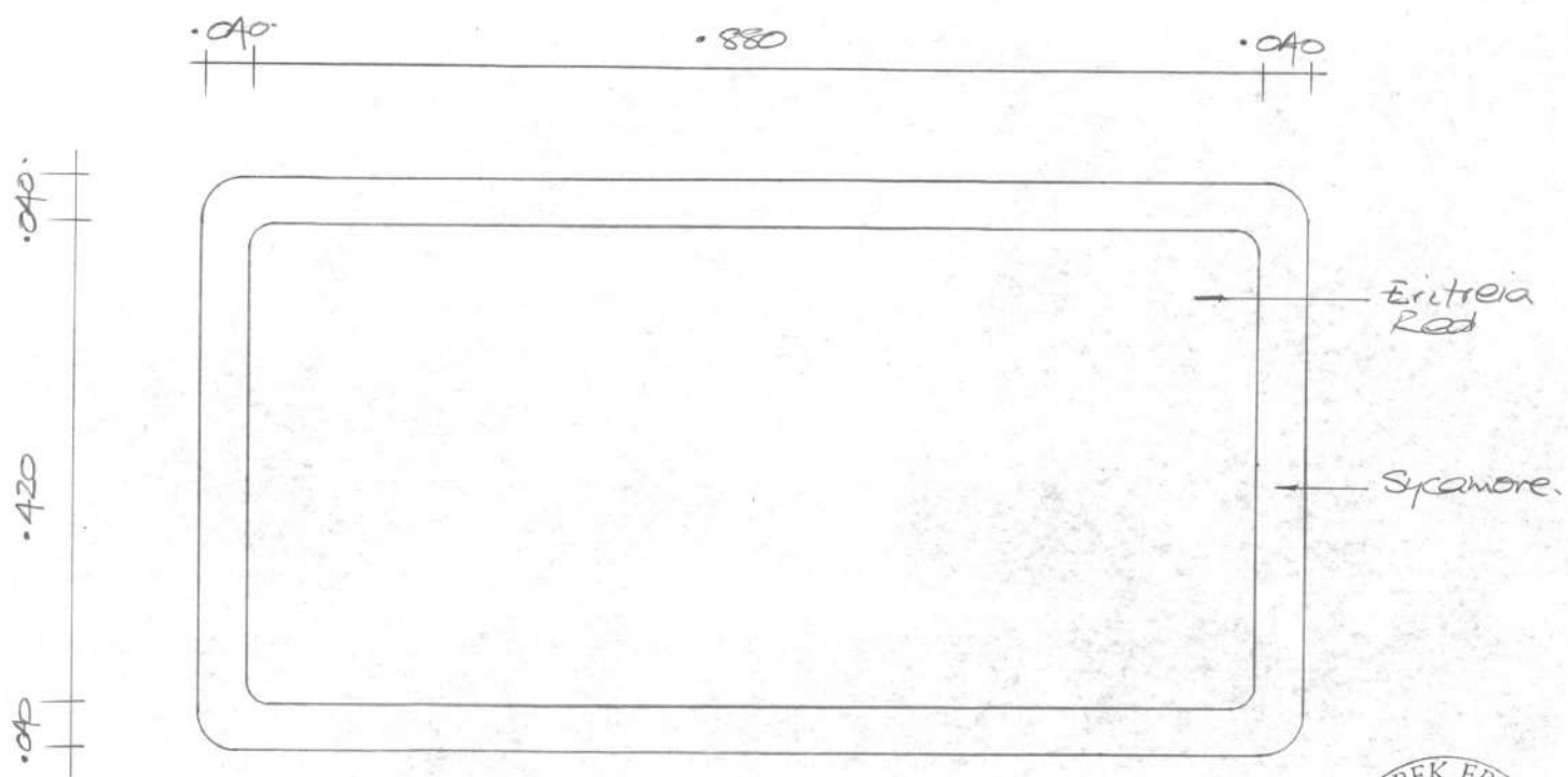
PLAN PAIR OF BEDSIDE CABINETS FOR MASTER BED ROOM BUTE.
