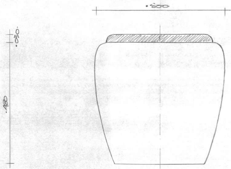
Side Elevation (Preferred Alternative)
