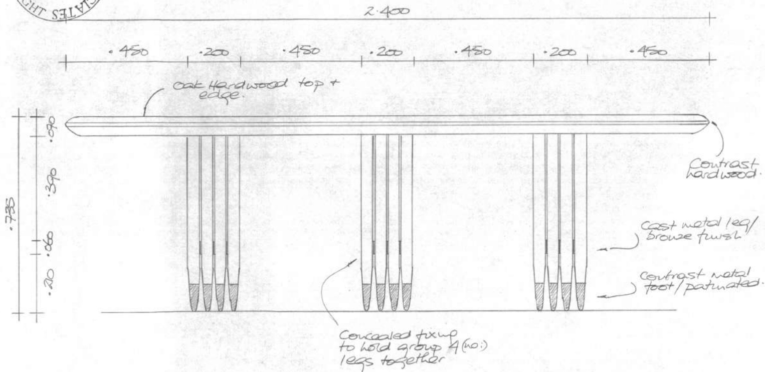
LONG ELEVATION DINING TABLE FOR BUTE HOUSE PROPOSED
