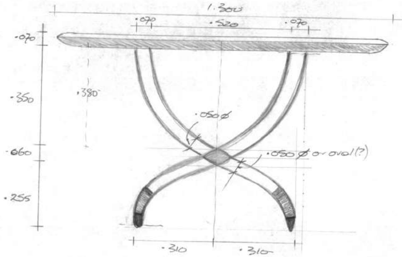
End Elevation - Dining Table for BUTE HOUSE
